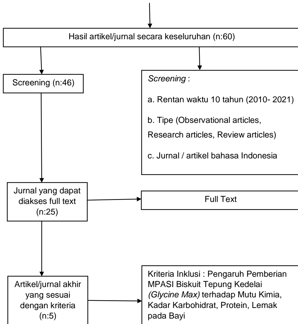
Gambar 1. Flow Chart
